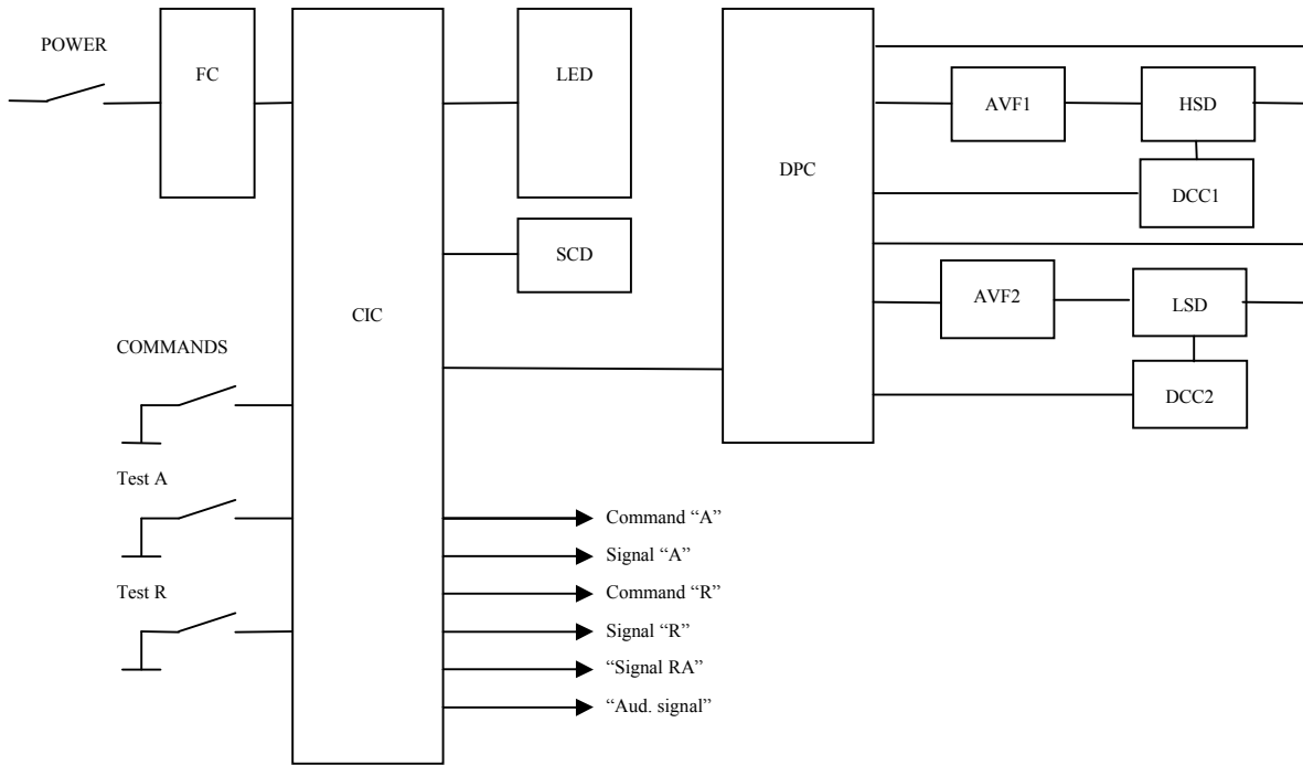
Figure 2 - Structure chart of the device
